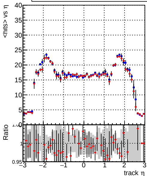
mean hits vs \eta — DQM_mkFit_TT_retrain — DQM_mkFit_TTold
