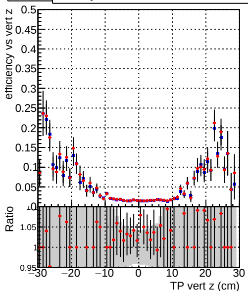
Efficiency vs. \text{TP vert } z
