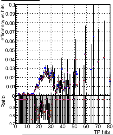
Efficiency vs hit Legend: DOM_mkFit_TT_retrain-lowpt DOM_mkFit_TT_NEWdefault_specPless1-lowpt DOM_mkFit_TT_NEWdefault_specPless2-lowpt DOM_mkFit_TT_NEWdefault_specPless3-lowpt DOM_mkFit_TT_NEWdefault_specPless4-lowpt
