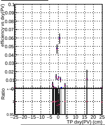
Efficiency vs Dxy(PV) DOM_mkFit_TT_retrain-lowpt DOM_mkFit_TT_NEWdefault_specPless1-lowpt DOM_mkFit_TT_NEWdefault_specPless2-lowpt DOM_mkFit_TT_NEWdefault_specPless3-lowpt DOM_mkFit_TT_NEWdefault_specPless4-lowpt
