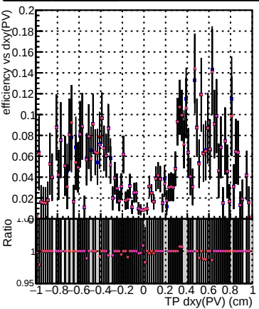
Efficiency vs Dxy(PV) DOM_mkFit_TT_retrain-lowpt DOM_mkFit_TT_NEWdefault_specPless1-lowpt DOM_mkFit_TT_NEWdefault_specPless2-lowpt DOM_mkFit_TT_NEWdefault_specPless3-lowpt DOM_mkFit_TT_NEWdefault_specPless4-lowpt
