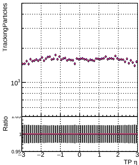
N of sim —▲— —●— —○— DOM mkFit TT NEWdefault specP Less2 owpt DOM mkFit TT NEWdefault specP Less3 owpt DOM mkFit TT NEWdefault specP Less4 owpt
