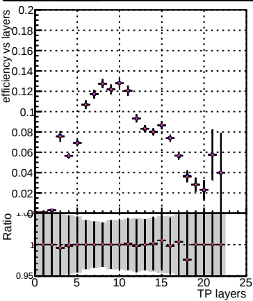
Efficiency vs hit DOM_mkFit_TT_retrain-lowpt DOM_mkFit_TT_NEWdefault_specPless1-lowpt DOM_mkFit_TT_NEWdefault_specPless2-lowpt DOM_mkFit_TT_NEWdefault_specPless3-lowpt DOM_mkFit_TT_NEWdefault_specPless4-lowpt
