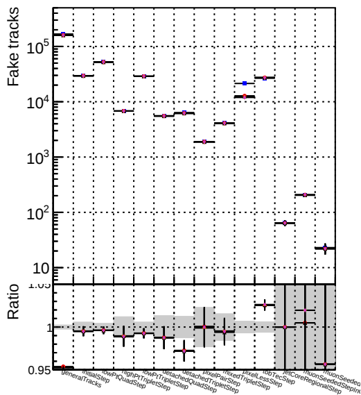
Number Symbol Model Method Dataset Configuration Performance 1 Red Star DOM mkFit TT NEWdefault specPLess2-lowpt 2 Black Star DOM mkFit TT NEWdefault specPLess3-lowpt 3 Orange Star DOM mkFit TT NEWdefault specPLess4-lowpt
