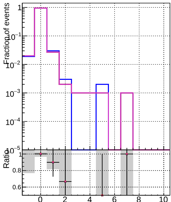
TruePVLocationIndexInRecoVertexCollection
