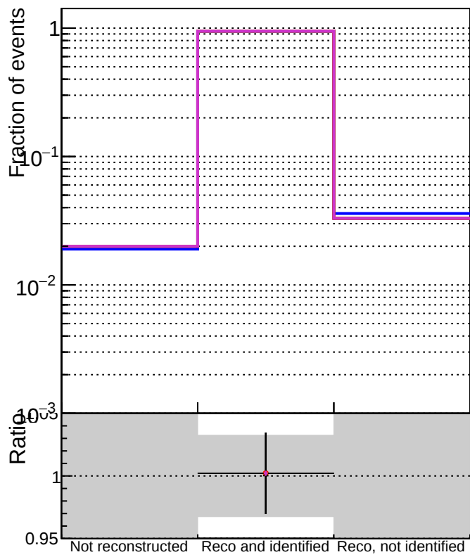
TruePVLocationIndexInRecoVertexCollectionCumulative
