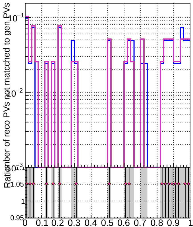
RecoPVAssoc2GenPVnotmatched_missing
