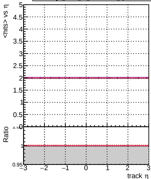
Legend: DOM mkFit TT retain-lowpt (blue), DOM mkFit TT NEWdefault specPless1-lowpt (red), DOM mkFit TT NEWdefault specPless2-lowpt (orange), DOM mkFit TT NEWdefault specPless3-lowpt (purple), DOM mkFit TT NEWdefault specPless4-lowpt (pink). mean hits
