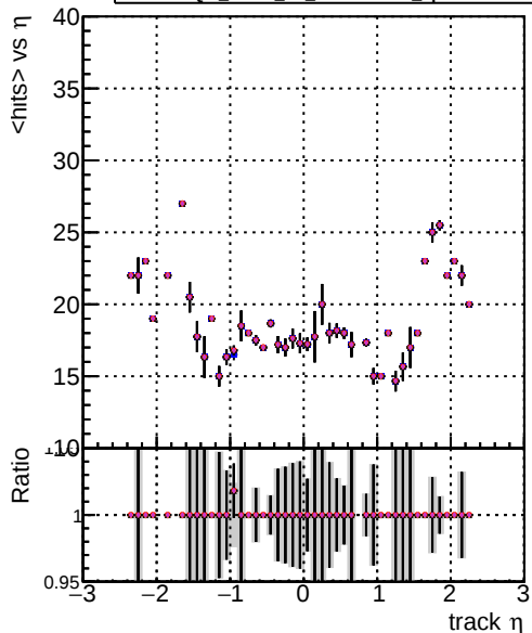
mean hit DOM mkFit TT retain_lowpt DOM mkFit TT NEWdefault specPless1_lowpt DOM mkFit TT NEWdefault specPless2_lowpt DOM mkFit TT NEWdefault specPless3_lowpt DOM mkFit TT NEWdefault specPless4_lowpt
