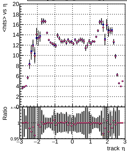
Legend for mean hits vs \eta : DOM mkFit TT (train-lowpt) DOM mkFit TT (NEWdefault specPless1-lowpt) DOM mkFit TT (NEWdefault specPless2-lowpt) DOM mkFit TT (NEWdefault specPless3-lowpt) DOM mkFit TT (NEWdefault specPless4-lowpt)
