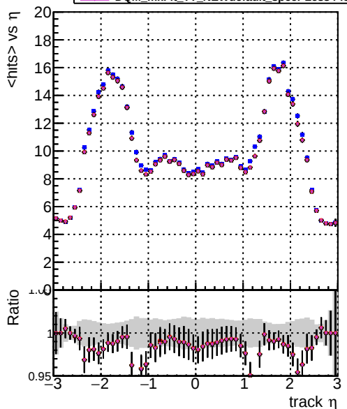
Legend: DOM mkFit TT (retail-lowpt), DOM mkFit TT NEWdefault specPless1-lowpt, DOM mkFit TT NEWdefault specPless2-lowpt, DOM mkFit TT NEWdefault specPless3-lowpt, DOM mkFit TT NEWdefault specPless4-lowpt mean hits
