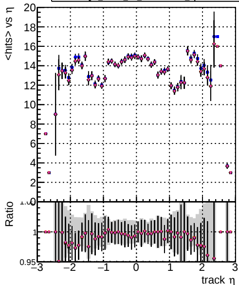
Legend for <math>\langle \text{hits} \rangle \text{ vs } \eta</math>: DOM mkFit TT (train) lowpt DOM mkFit TT NEWdefault specPless1-lowpt DOM mkFit TT NEWdefault specPless2-lowpt DOM mkFit TT NEWdefault specPless3-lowpt DOM mkFit TT NEWdefault specPless4-lowpt
