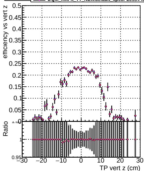
Efficiency vs. TP vert z (cm) DOM mkFit TT (train-lowpt) DOM mkFit TT (NEWdefault specPLess1-lowpt) DOM mkFit TT (NEWdefault specPLess2-lowpt) DOM mkFit TT (NEWdefault specPLess3-lowpt) DOM mkFit TT (NEWdefault specPLess4-lowpt)
