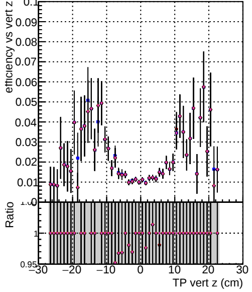
Efficiency vs vert z DOM mkFit TT retail-lowpt DOM mkFit TT NEWdefault specPless1-lowpt DOM mkFit TT NEWdefault specPless2-lowpt DOM mkFit TT NEWdefault specPless3-lowpt DOM mkFit TT NEWdefault specPless4-lowpt
