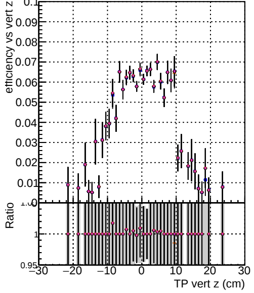
Efficiency vs. sim PV z DOM mkFit NEWdefault specPLess1-lowpt DOM mkFit NEWdefault specPLess2-lowpt DOM mkFit NEWdefault specPLess3-lowpt DOM mkFit NEWdefault specPLess4-lowpt
