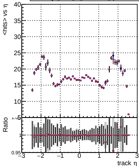
Legend for mean hits vs \eta : DOM mkFit TT (train-lowpt) DOM mkFit TT (NEWdefault specPless1-lowpt) DOM mkFit TT (NEWdefault specPless2-lowpt) DOM mkFit TT (NEWdefault specPless3-lowpt) DOM mkFit TT (NEWdefault specPless4-lowpt)
