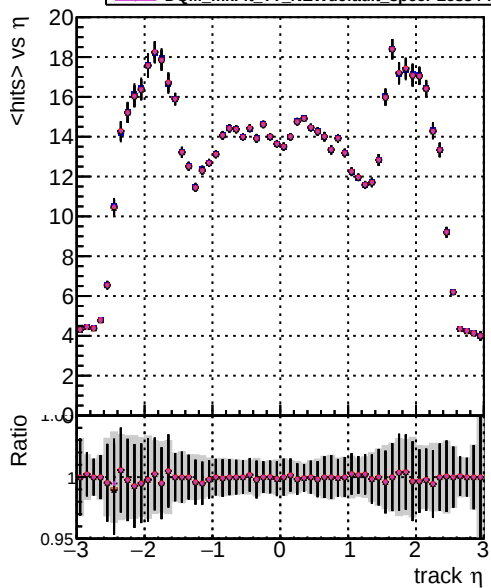
Legend for mean hits vs track \eta : DOM mkFit TT NEWdefault specPless1-lowpt DOM mkFit TT NEWdefault specPless2-lowpt DOM mkFit TT NEWdefault specPless3-lowpt DOM mkFit TT NEWdefault specPless4-lowpt
