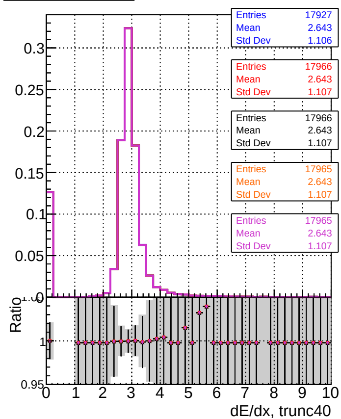
DOM_mkFit TT_retrain-lowpt DOM_mkFit TT_NEWdefault_specPless1-lowpt DOM_mkFit TT_NEWdefault_specPless2-lowpt DOM_mkFit TT_NEWdefault_specPless3-lowpt DOM_mkFit TT_NEWdefault_specPless4-lowpt
