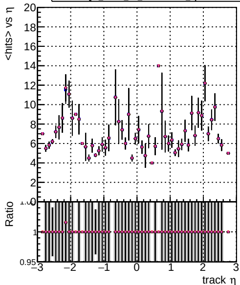
mean hit DOM mkFit TT NEWdefault specPless1-lowpt DOM mkFit TT NEWdefault specPless2-lowpt DOM mkFit TT NEWdefault specPless3-lowpt DOM mkFit TT NEWdefault specPless4-lowpt
