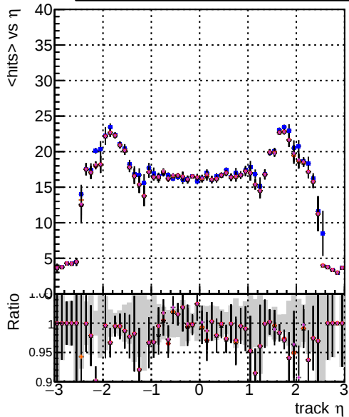
Legend: DQM mkFit TT (train-lowpt), DQM mkFit TT (NEWdefault specPless1-lowpt), DQM mkFit TT (NEWdefault specPless2-lowpt), DQM mkFit TT (NEWdefault specPless3-lowpt), DQM mkFit TT (NEWdefault specPless4-lowpt) mean hits
