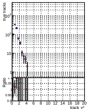
N of reco track vs. \chi^2 for different detector regions
