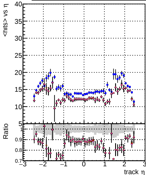
mean hit DOM mkFit TT retail-lowpt DOM mkFit TT NEWdefault specPless1-lowpt DOM mkFit TT NEWdefault specPless2-lowpt DOM mkFit TT NEWdefault specPless3-lowpt DOM mkFit TT NEWdefault specPless4-lowpt
