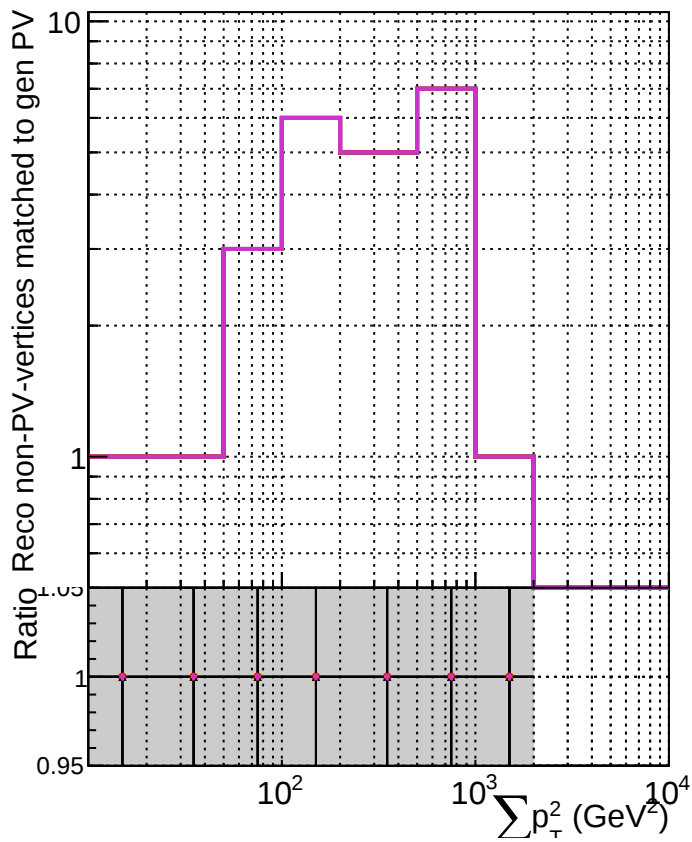
RecoAssoc2GenPVMatchedNotHighest_Pt2
