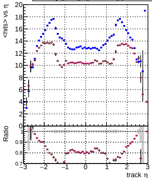
Legend for mean hits vs \eta : DOM mkFit TT (train-lowpt) DOM mkFit TT NEWdefault specPless1-lowpt DOM mkFit TT NEWdefault specPless2-lowpt DOM mkFit TT NEWdefault specPless3-lowpt DOM mkFit TT NEWdefault specPless4-lowpt
