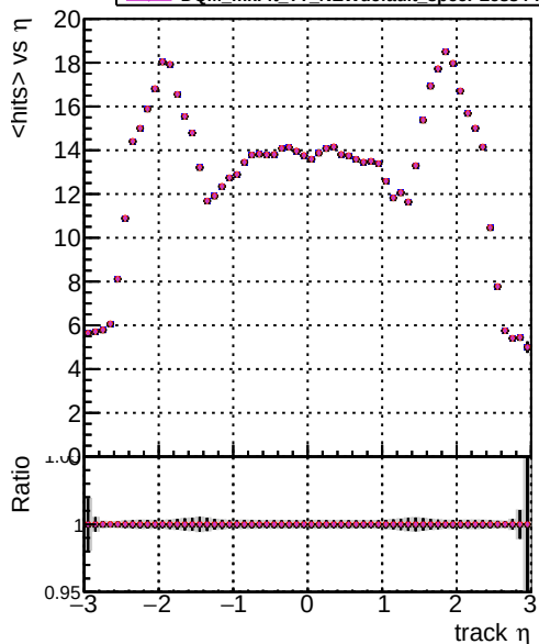
mean hits vs \eta DOM mkFit TT retain-lowpt DOM mkFit TT NEWdefault specPLess1-lowpt DOM mkFit TT NEWdefault specPLess2-lowpt DOM mkFit TT NEWdefault specPLess3-lowpt DOM mkFit TT NEWdefault specPLess4-lowpt
