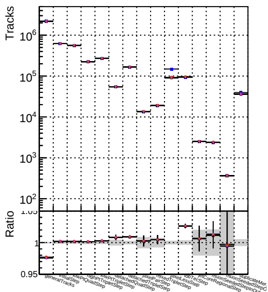
Number of tracks vs collection DOM mkFit TT retain-lowpt specPless1-lowpt DOM mkFit TT NEWdefault specPless2-lowpt DOM mkFit TT NEWdefault specPless3-lowpt DOM mkFit TT NEWdefault specPless4-lowpt
