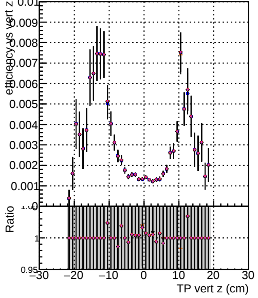
Efficiency vs. TP vert z (cm) DOM mkFit TT retail-lowpt DOM mkFit TT NEWdefault specPless1-lowpt DOM mkFit TT NEWdefault specPless2-lowpt DOM mkFit TT NEWdefault specPless3-lowpt DOM mkFit TT NEWdefault specPless4-lowpt
