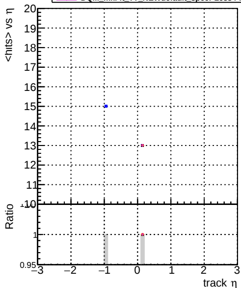
mean hits DOM mkFit TT retain-lowpt DOM mkFit TT NEWdefault specPLess1-lowpt DOM mkFit TT NEWdefault specPLess2-lowpt DOM mkFit TT NEWdefault specPLess3-lowpt DOM mkFit TT NEWdefault specPLess4-lowpt
