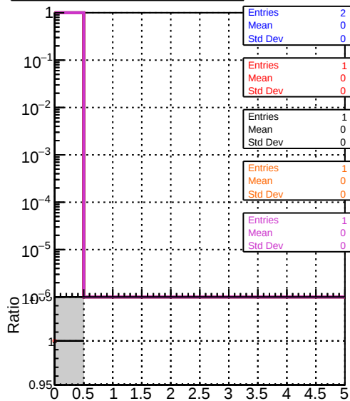
mean hits DOM mkFit TT retain-lowpt DOM mkFit TT NEWdefault specPLess1-lowpt DOM mkFit TT NEWdefault specPLess2-lowpt DOM mkFit TT NEWdefault specPLess3-lowpt DOM mkFit TT NEWdefault specPLess4-lowpt
