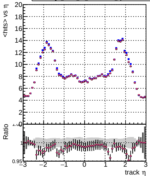
Legend for mean hits vs \eta : DOM mkFit TT (blue) DOM mkFit TT NEWdefault specPless1-lowpt (red) DOM mkFit TT NEWdefault specPless2-lowpt (green) DOM mkFit TT NEWdefault specPless3-lowpt (orange) DOM mkFit TT NEWdefault specPless4-lowpt (purple)
