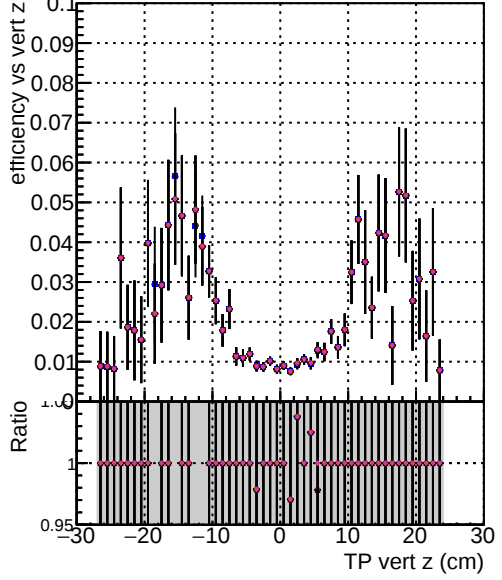
Efficiency vs. TP vert z (cm) DOM mkFit TT train-lowpt DOM mkFit NEWdefault specPLess1-lowpt DOM mkFit NEWdefault specPLess2-lowpt DOM mkFit NEWdefault specPLess3-lowpt DOM mkFit NEWdefault specPLess4-lowpt
