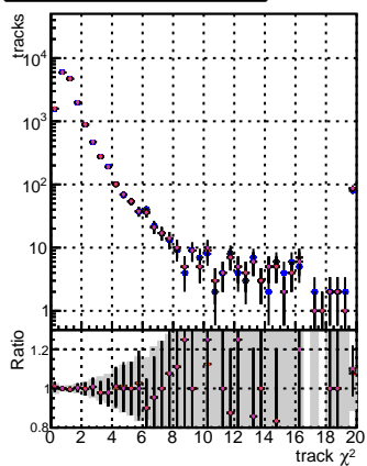
N of reco track vs. \chi^2 for different detector components
