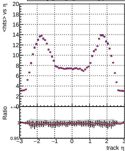
Legend: DOM mkFit TT retain-lowpt, DOM mkFit TT NEWdefault specPless1-lowpt, DOM mkFit TT NEWdefault specPless2-lowpt, DOM mkFit TT NEWdefault specPless3-lowpt, DOM mkFit TT NEWdefault specPless4-lowpt mean hit
