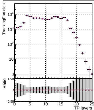
N of sim —●— DQM_mkFit_TT_NEWdefault_specPLess3-lowpt —●— DQM_mkFit_TT_NEWdefault_specPLess4-lowpt
