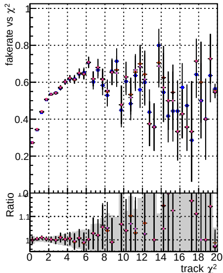
Fake rate vs. DOM mkt fit TT retrain lowpt other
