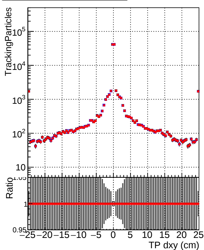
N of simulated track Legend: DQM_mkFit_TT_retrain-lowpt (grey square) DQM_mkFit_TTold-lowpt (red circle)
