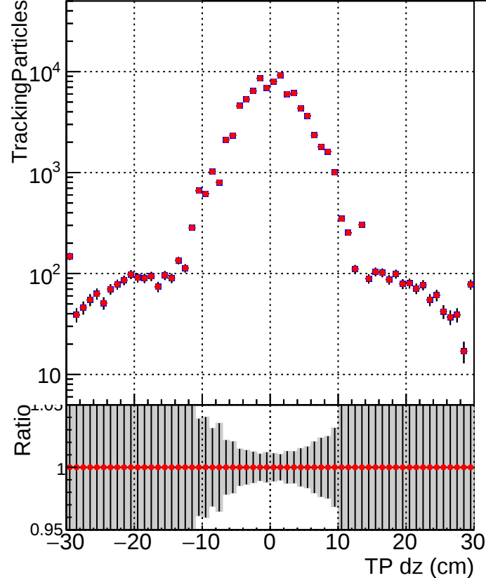
N of simulated track Legend: DQM_mkFit_TT_retrain-lowpt (grey square) DQM_mkFit_TTold-lowpt (red circle)
