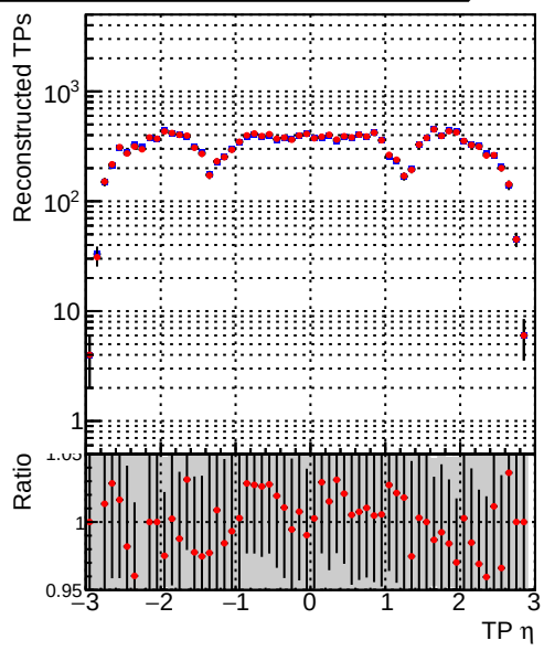
Legend: \bullet DQM_mkFit_TT_retrain-lowpt \bullet DQM_mkFit_TTold-lowpt
