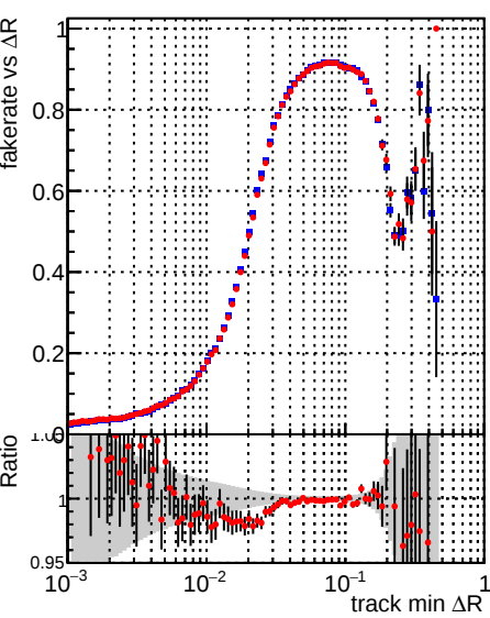
Fake rate vs \Delta R(\text{track, jet}) Legend: DQM_mkFit_TT_retrain-lowpt (blue line with error bars) DQM_mkFit_TTold-lowpt (red line with error bars)
