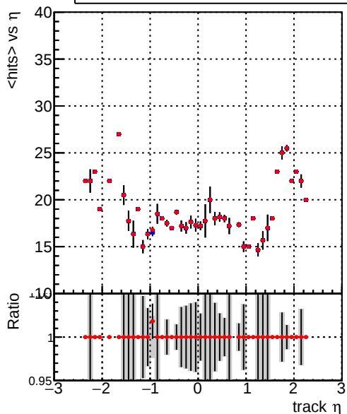
mean hit — DQM_mkFit_TT_retrain-lowpt — DQM_mkFit_TTold-lowpt
