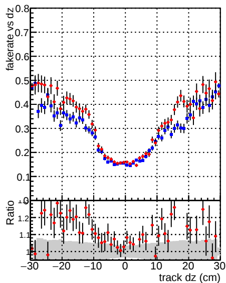
Fake rate vs dz —●— DQM_mkFit_TT_retrain-lowpt —●— DQM_mkFit_TTold-lowpt
