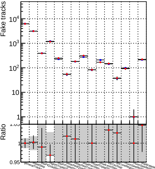
Number —●— DQM_mkFit_TTold-lowpt
