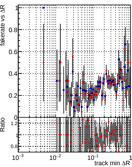
Fake rate vs \Delta R(\text{track, jet}) Legend: —■— DQM_mkFit_TT_retrain-lowpt —●— DQM_mkFit_TTold-lowpt
