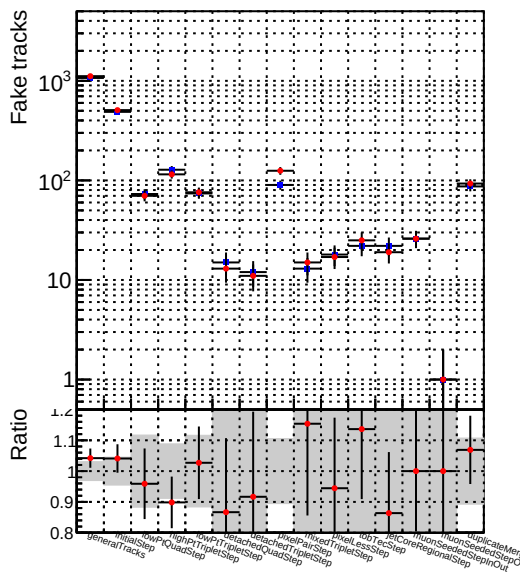
Number —●— DQM_mkFit_TTold-lowpt
