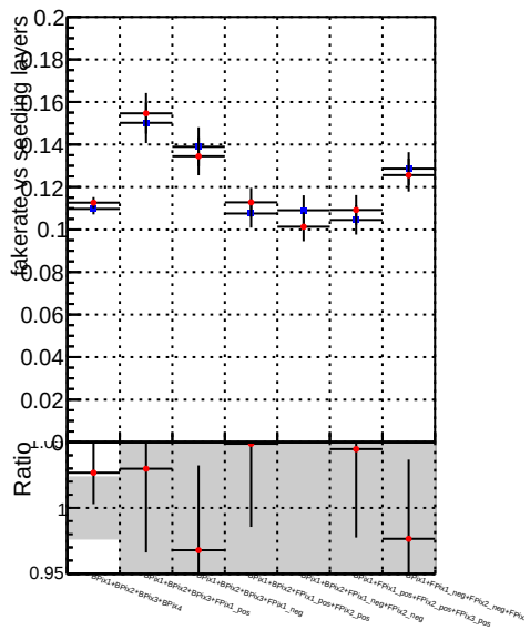
Fake rate vs. —●— DQM_mkFit_TT_retrain-lowpt —●— DQM_mkFit_TTold-lowpt
