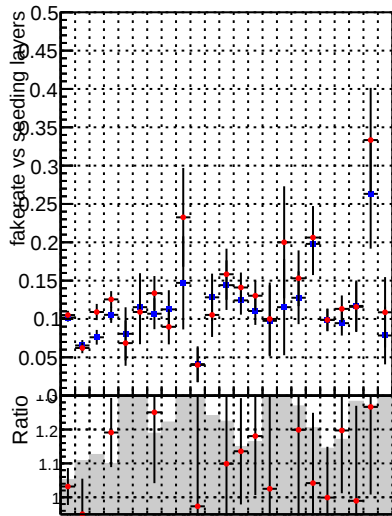
Fake rate vs. —●— DQM_mkFit_TT_retrain-lowpt —●— DQM_mkFit_TTold-lowpt
