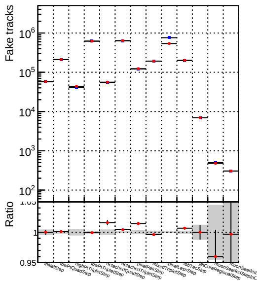
Number —●— DQM_mkFit_TTold-lowp
