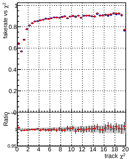
Fake rate vs. \chi^2 — DQM_mkFit_TT_retrain-lowpt — DQM_mkFit_TTold-lowpt
