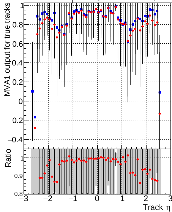
MVA1 of associated tracks (recoToSim) vs. track \eta Legend: DQM_mkFit_TT_retrain-lowpt (blue squares) DQM_mkFit_TTold-lowpt (red circles)
