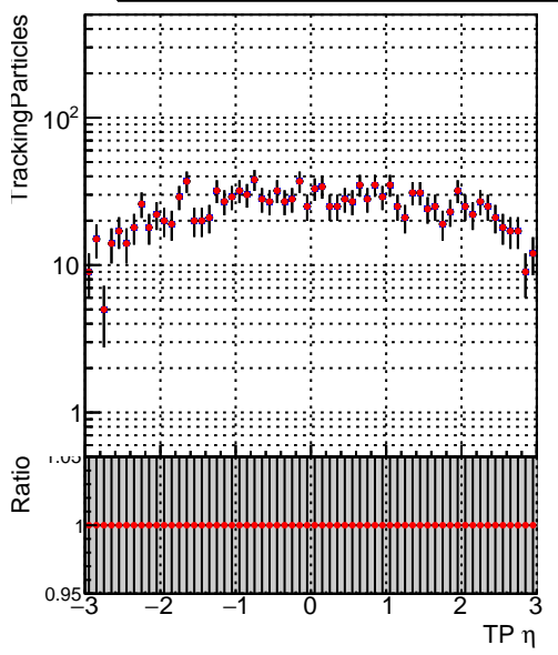
N of simulated tracks vs \eta Legend: - \blacksquare DQM_mkFit_TT_retrain-lowpt - \bullet DQM_mkFit_TTold-lowpt
